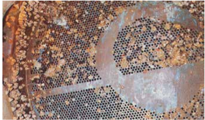
BEFORE — TYPICAL FOULING CONDENSER TUBE PLATE
